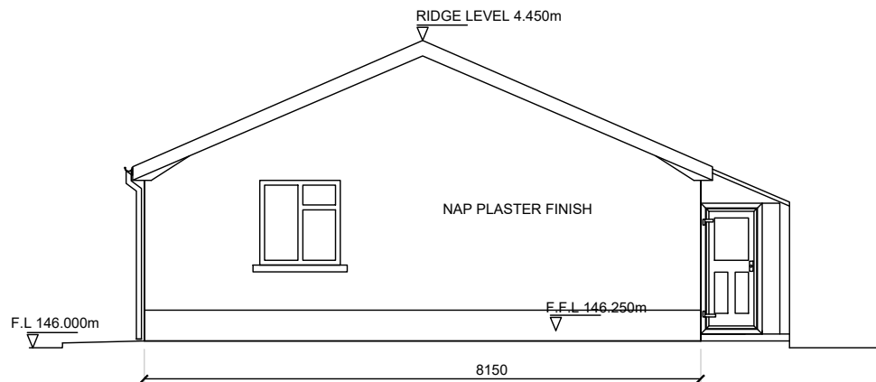
SIDE ELEVATION - WEST FACING SCALE; 1:100
