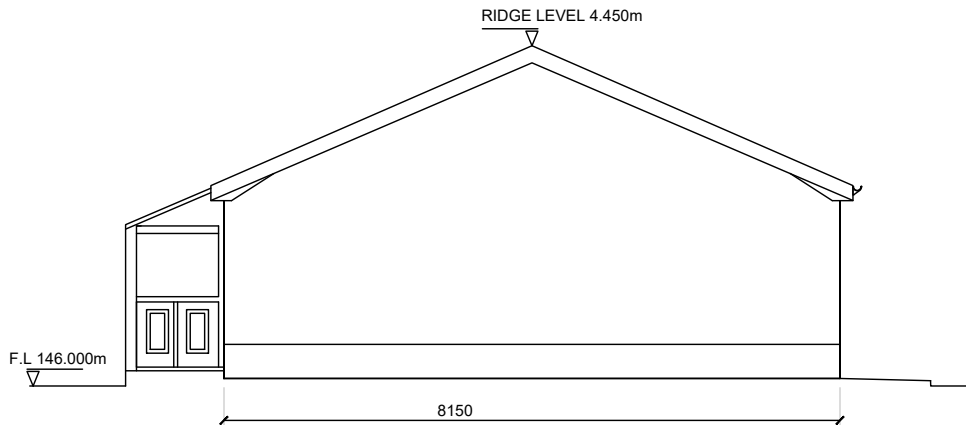
SIDE ELEVATION - EAST FACING SCALE; 1:100
