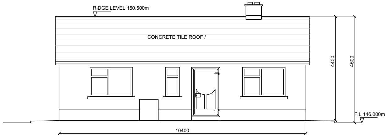
REAR ELEVATION - NORTH FACING SCALE; 1:100
