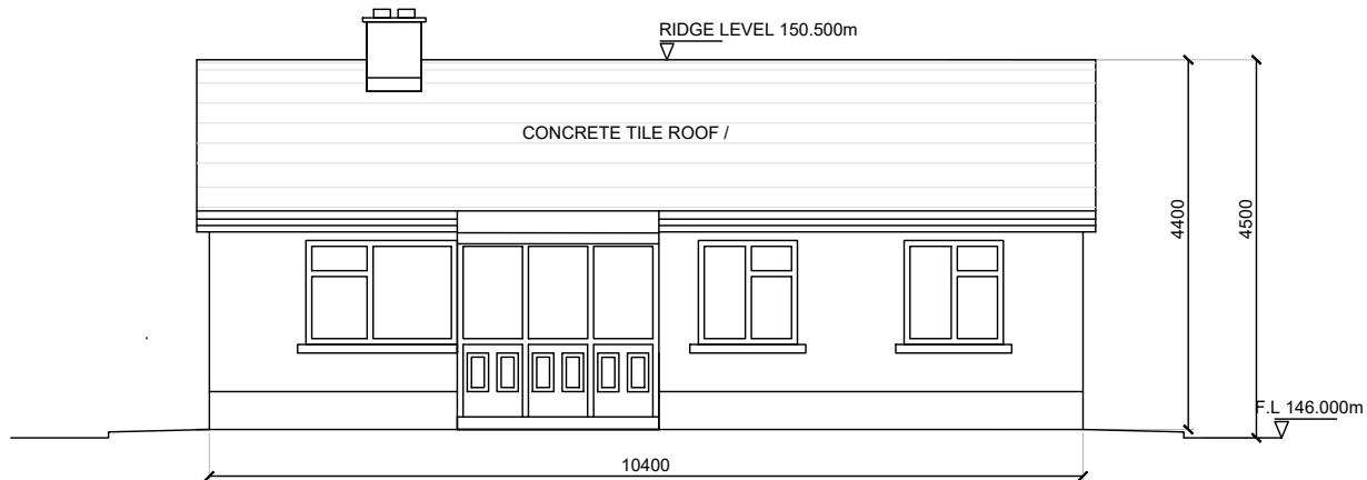
FRONT ELEVATION - SOUTH FACING SCALE; 1:100
